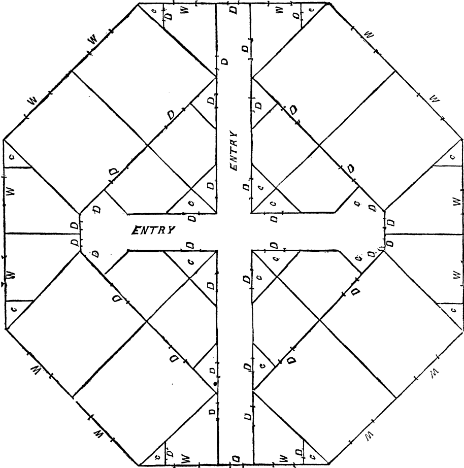
Fig. 21.—Second story of the 32-foot Octagon.
