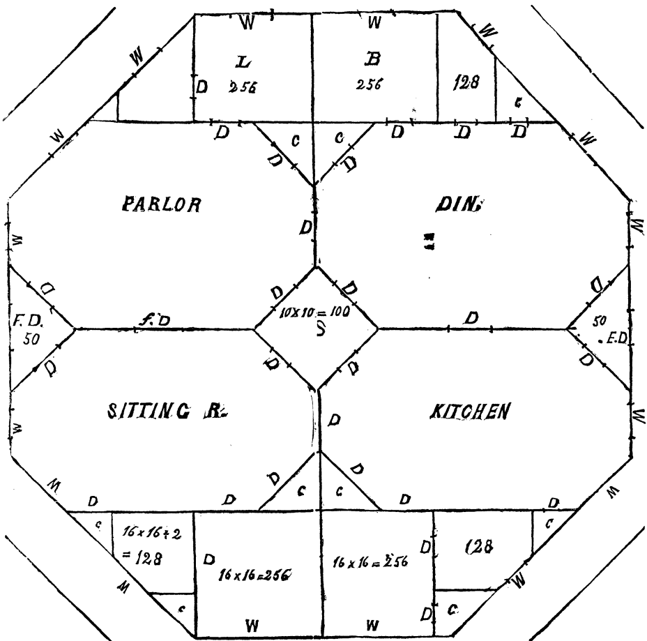
Fig. 20.—32-foot Octagon, main story.
