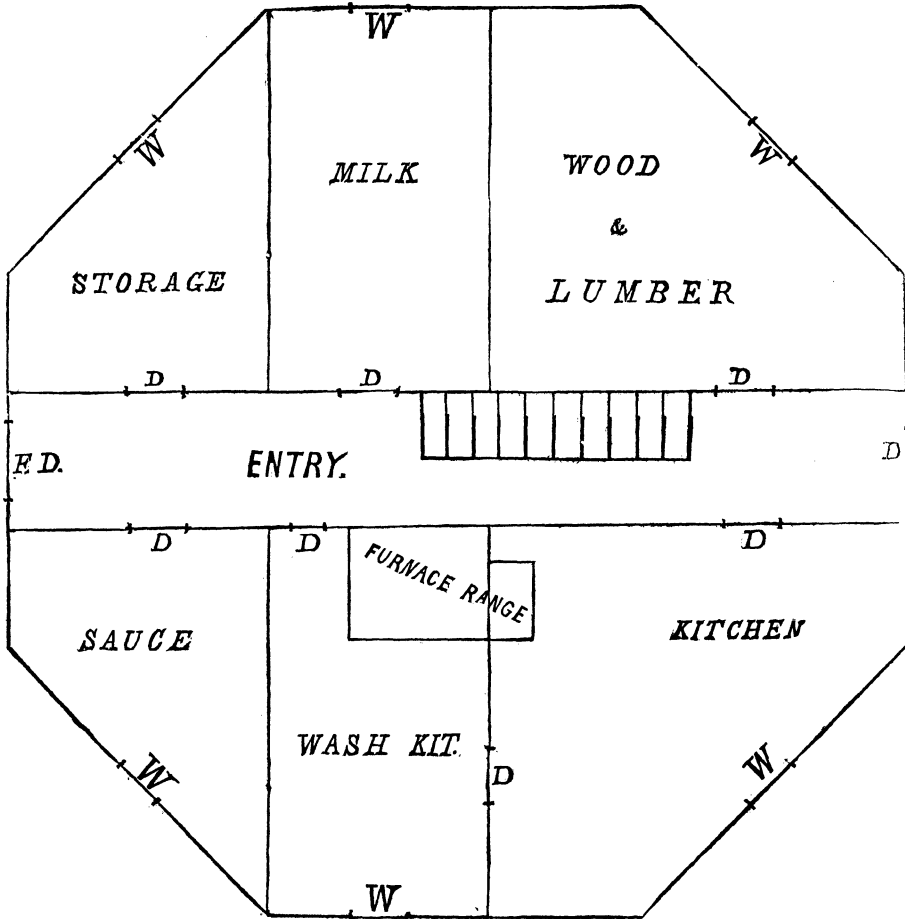
Fig. 11. The Octagon Basement.
