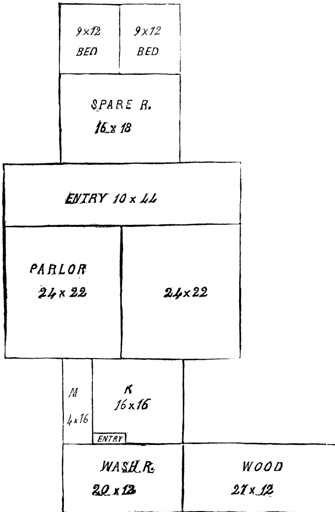
Fig. 18—Winged house, 32 by 42.
